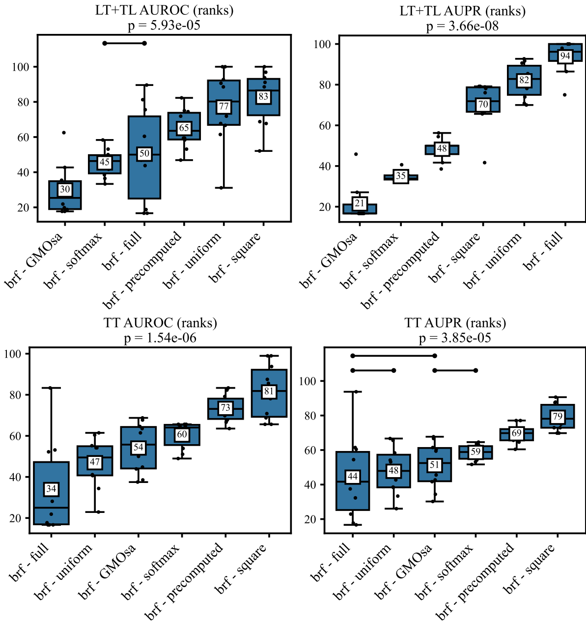
Figure 10 – Comparison of bipartite random forests for different prototype strategies. An omnibus p-value is obtained through a Friedman test and indicated below the title of each subfigure. We then perform pairwise Wilcoxon rank-sum tests as a post-hoc analysis. Estimators that could not be significantly distinguished from each other ( p > 0.05 ) are connected by cross-bars above their respective boxes. The pairwise test results are corrected by the Benjamini-Hochberg procedure (4, 5) in each subfigure. All pairwise comparisons are considered for the correction, even if not visible in the plot. See Section 2.8 for further description of the evaluation procedure.
